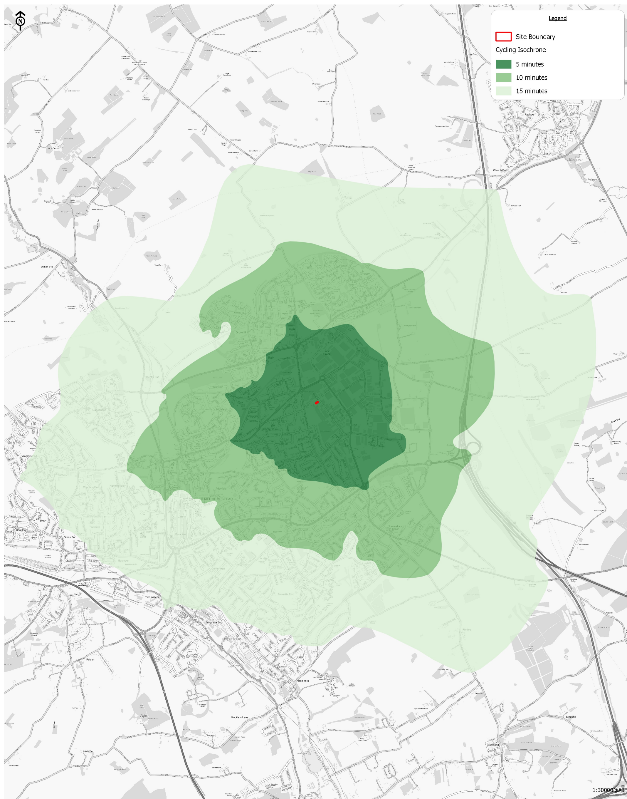
Figure 3: Cycling Isochrone
